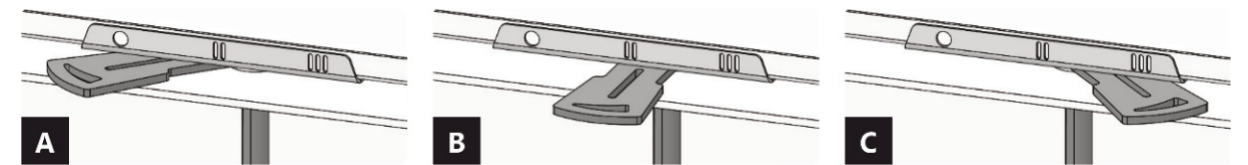
Fig. 7 Air intake controller – type 3
